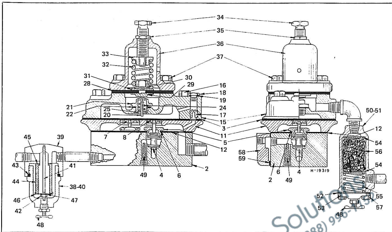
TYPE UFD-3 FREE AIR REGULATOR PARTS 7" STROKE UNITS
